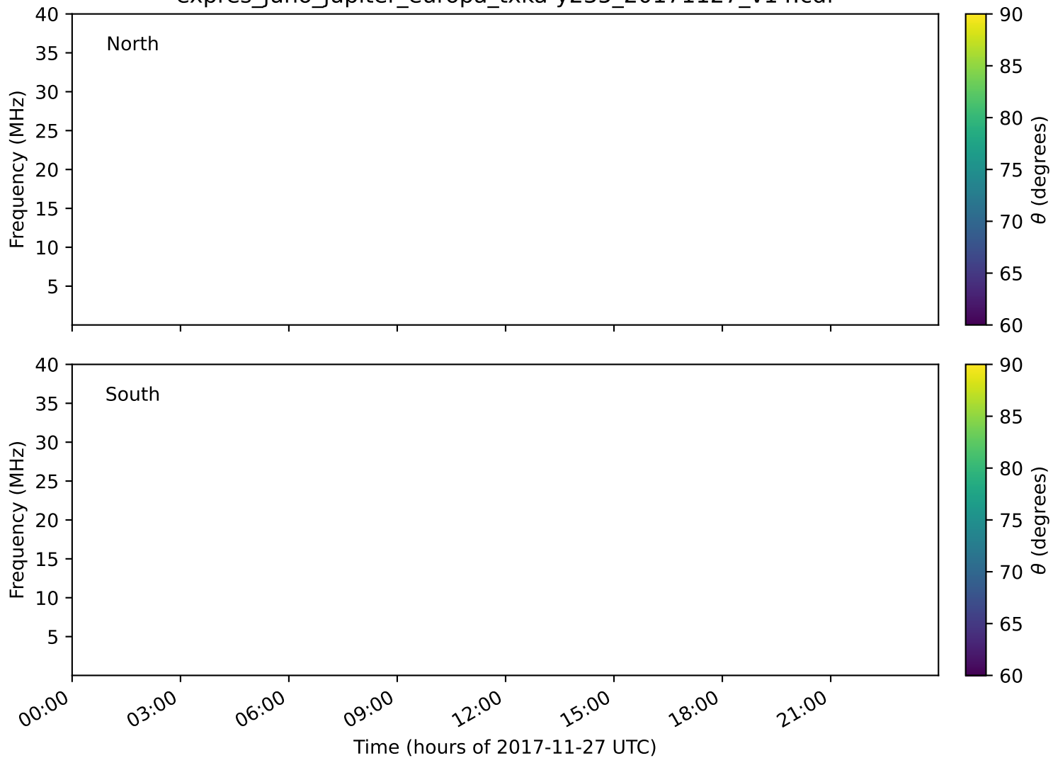
expres_juno_jupiter_europa_txka-y235_20171127_v14.cdf
