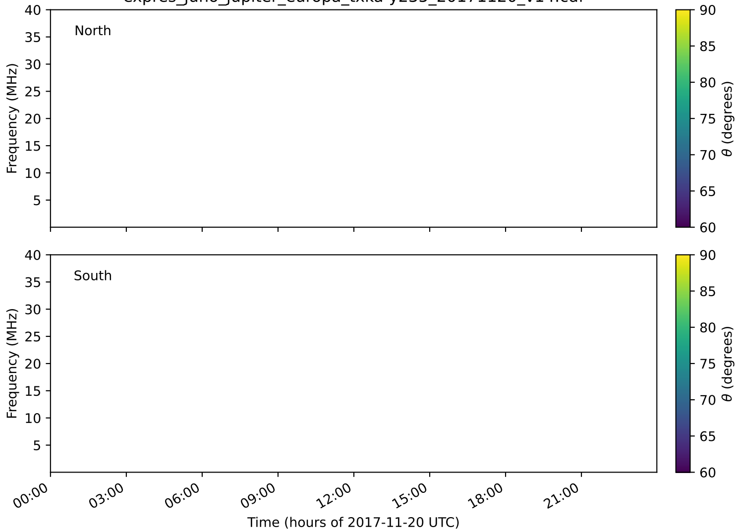
expres_juno_jupiter_europa_txka-y235_20171120_v14.cdf
