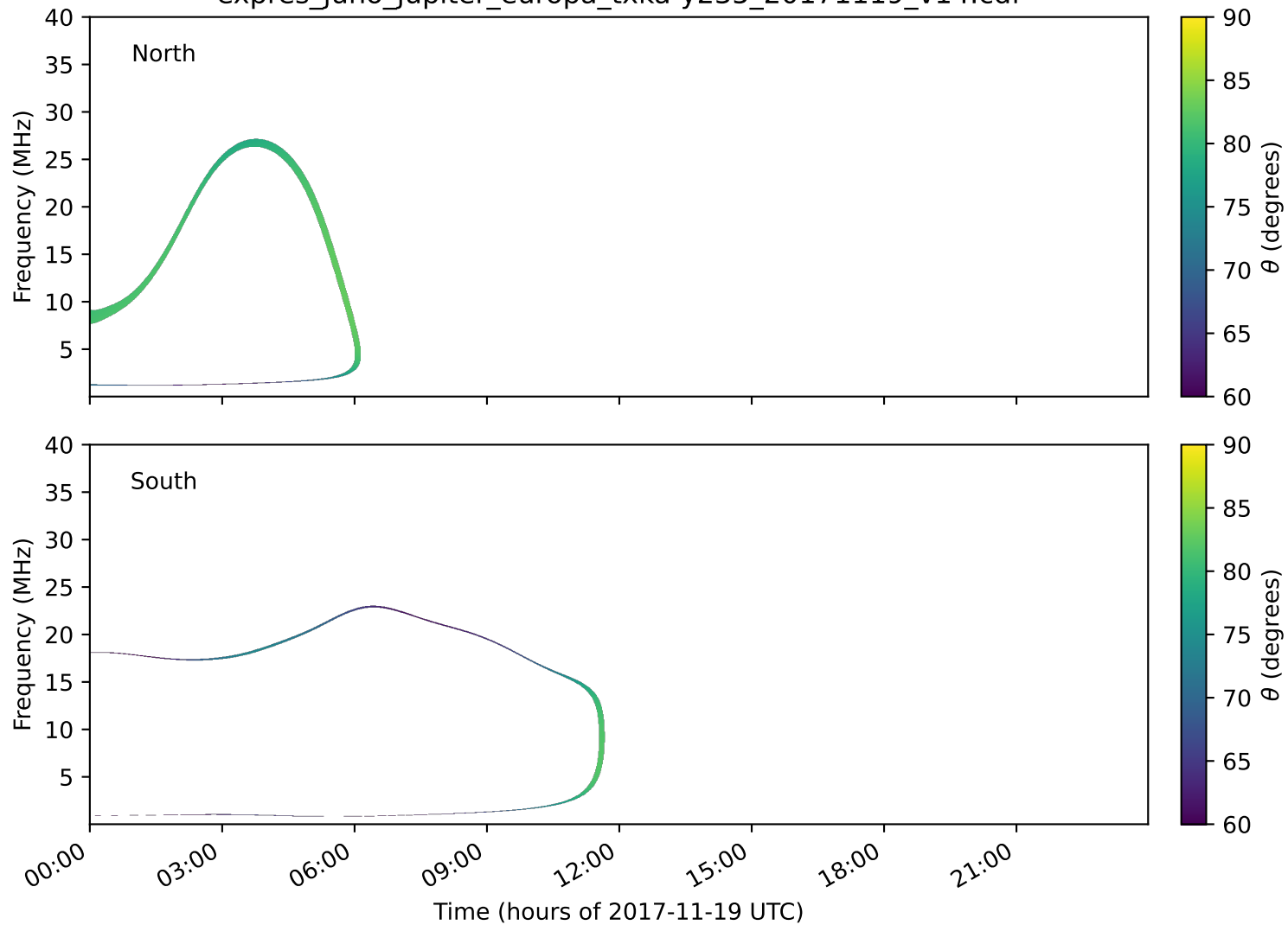
expres_juno_jupiter_europa_txka-y235_20171119_v14.cdf
