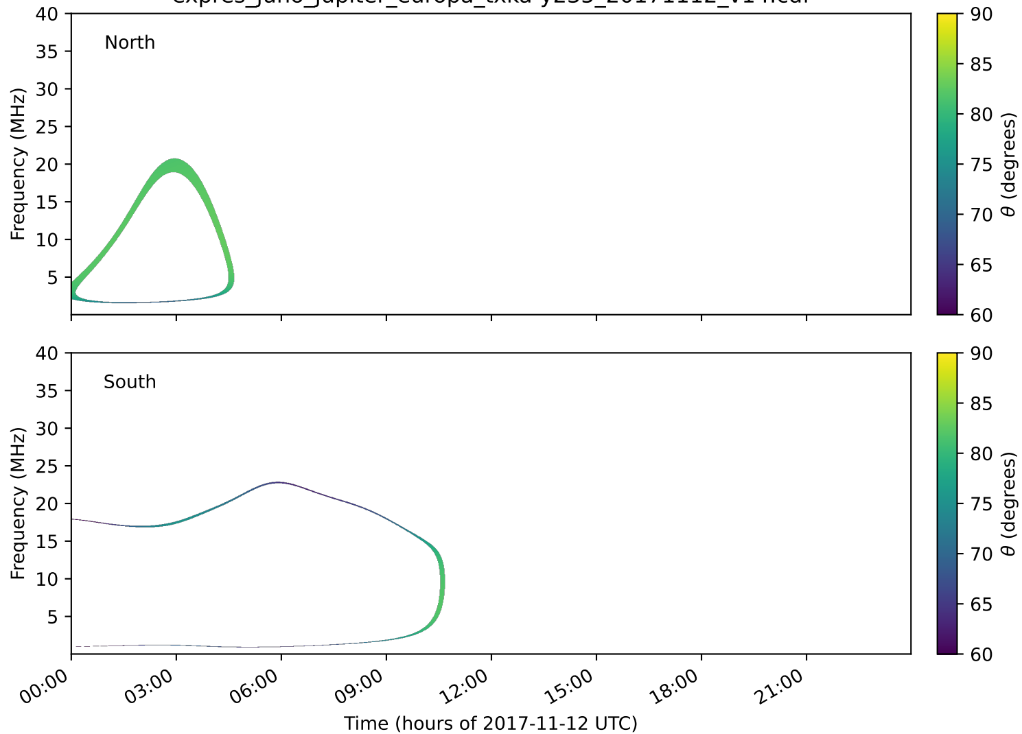
expres_juno_jupiter_europa_txka-y235_20171112_v14.cdf
