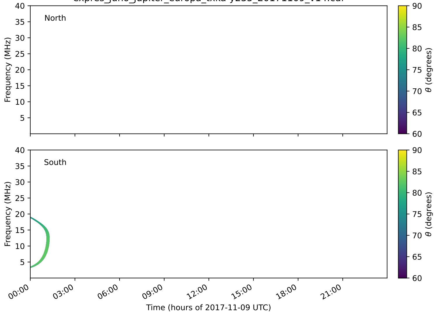
expres_juno_jupiter_europa_txka-y235_20171109_v14.cdf
