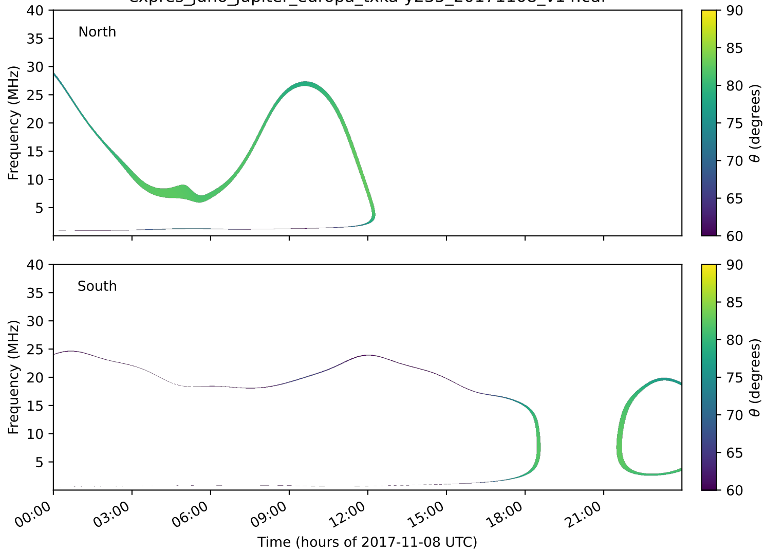
expres_juno_jupiter_europa_txka-y235_20171108_v14.cdf
