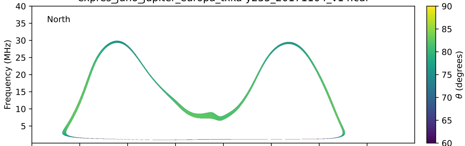
expres_juno_jupiter_europa_txka-y235_20171104_v14.cdf
