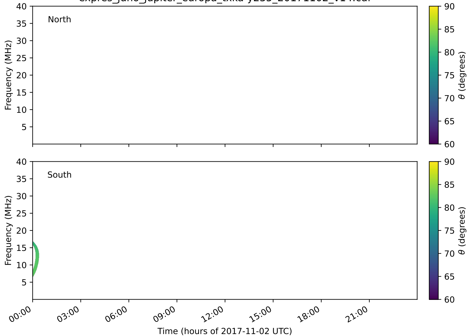
expres_juno_jupiter_europa_txka-y235_20171102_v14.cdf
