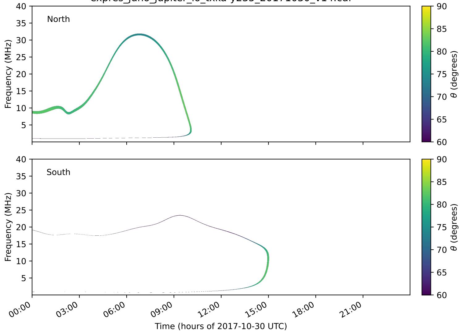
expres_juno_jupiter_io_txka-y235_20171030_v14.cdf
