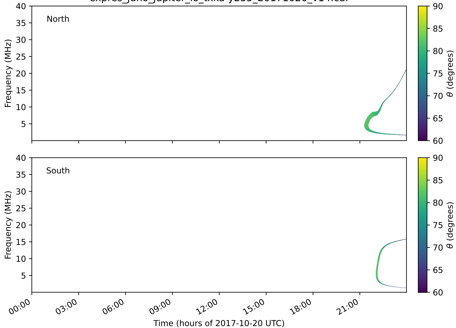
expres_juno_jupiter_io_txka-y235_20171020_v14.cdf
