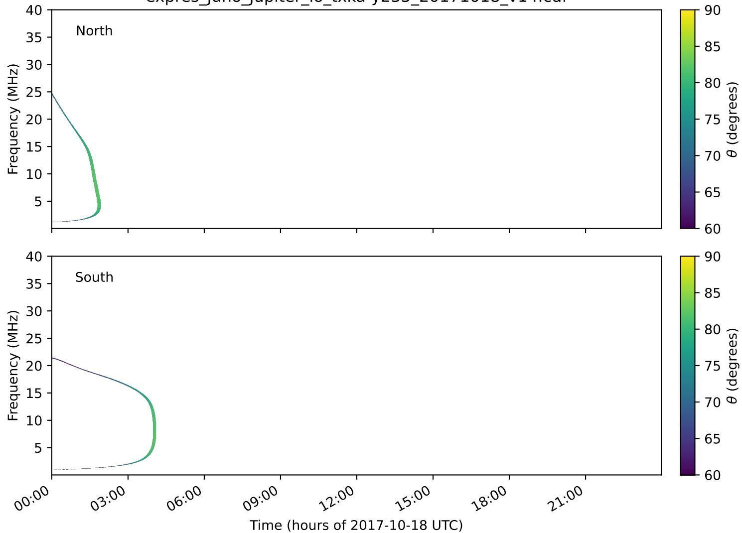
expres_juno_jupiter_io_txka-y235_20171018_v14.cdf
