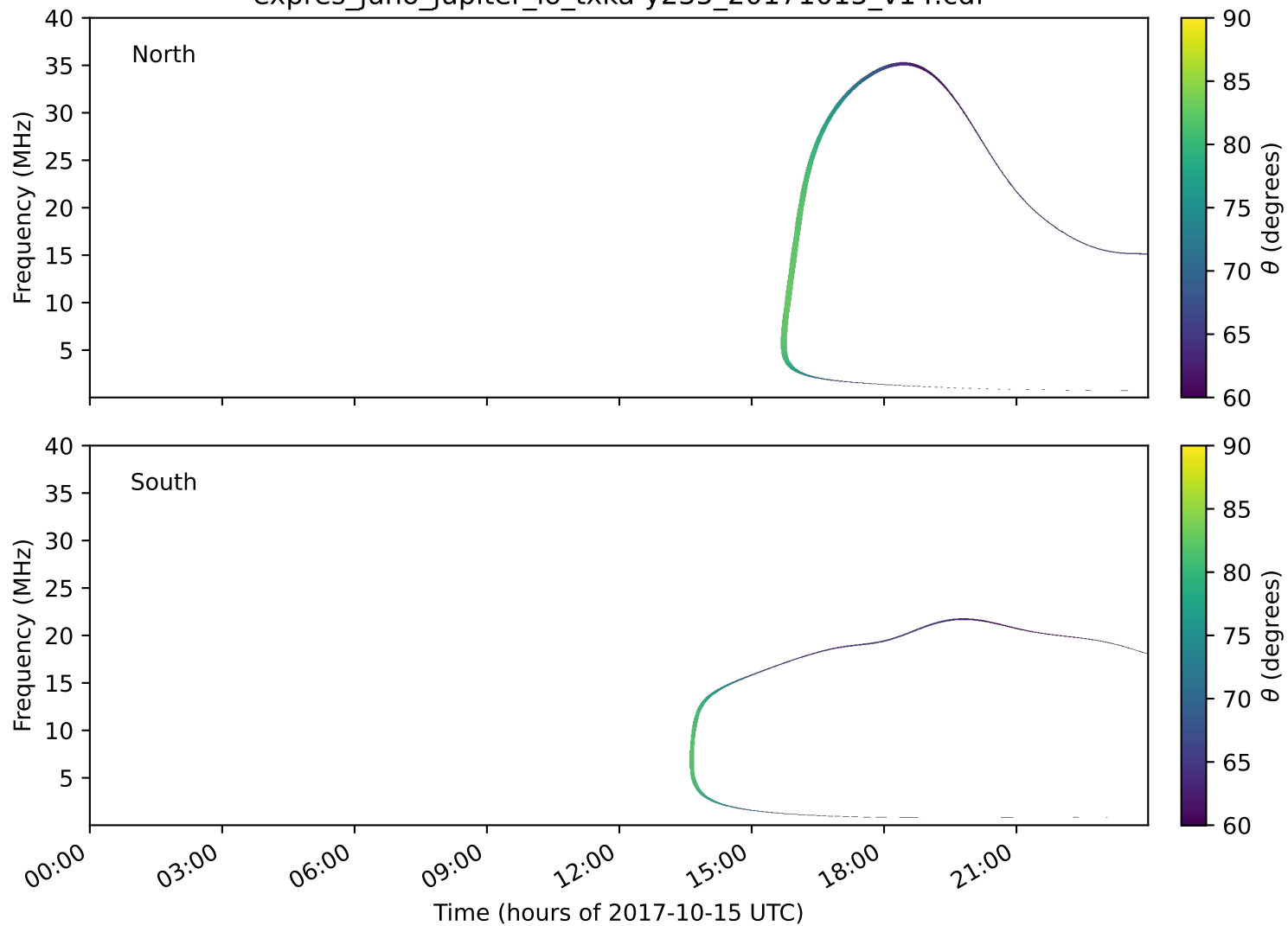
expres_juno_jupiter_io_txka-y235_20171015_v14.cdf
