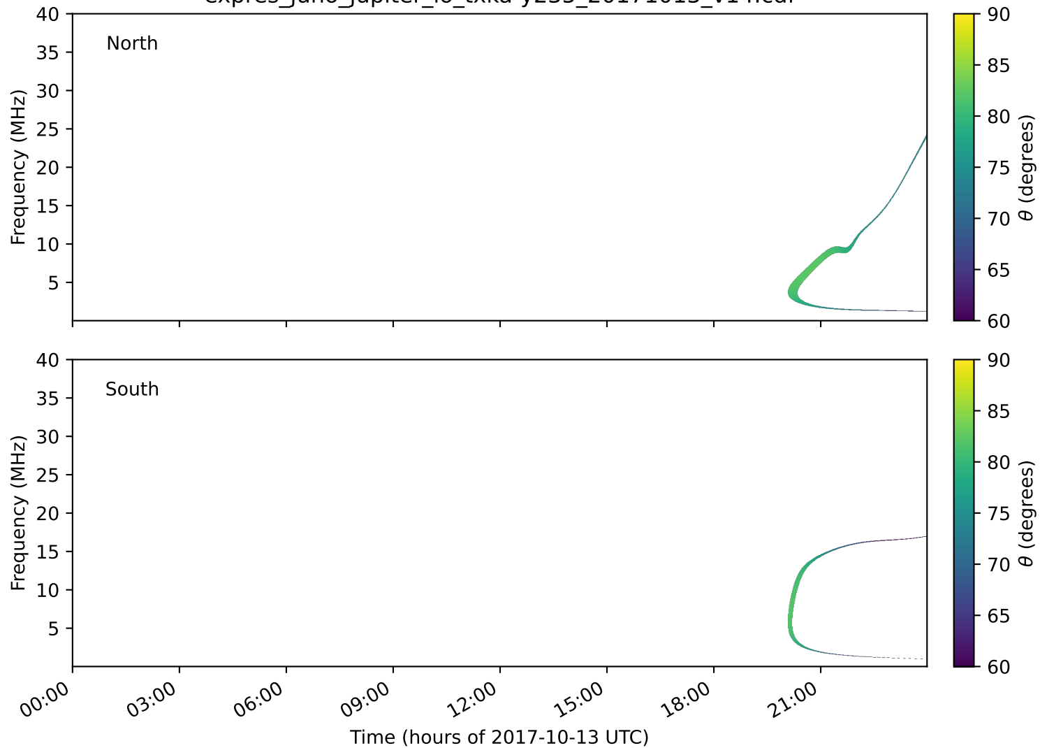
expres_juno_jupiter_io_txka-y235_20171013_v14.cdf
