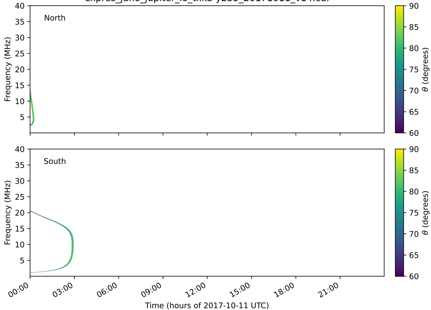
expres_juno_jupiter_io_txka-y235_20171011_v14.cdf
