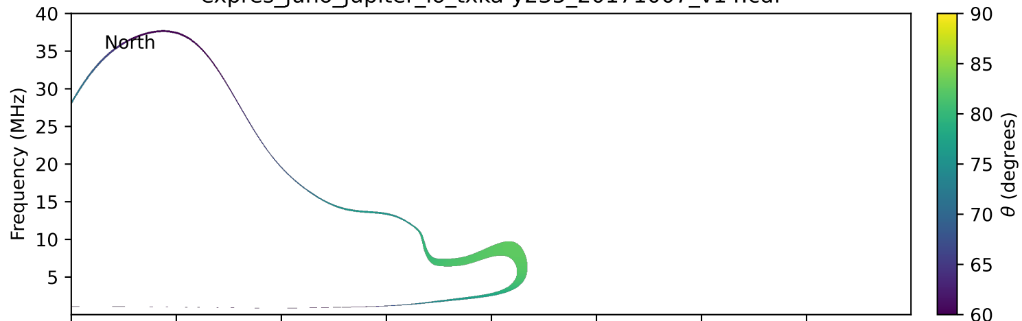
expres_juno_jupiter_io_txka-y235_20171007_v14.cdf
