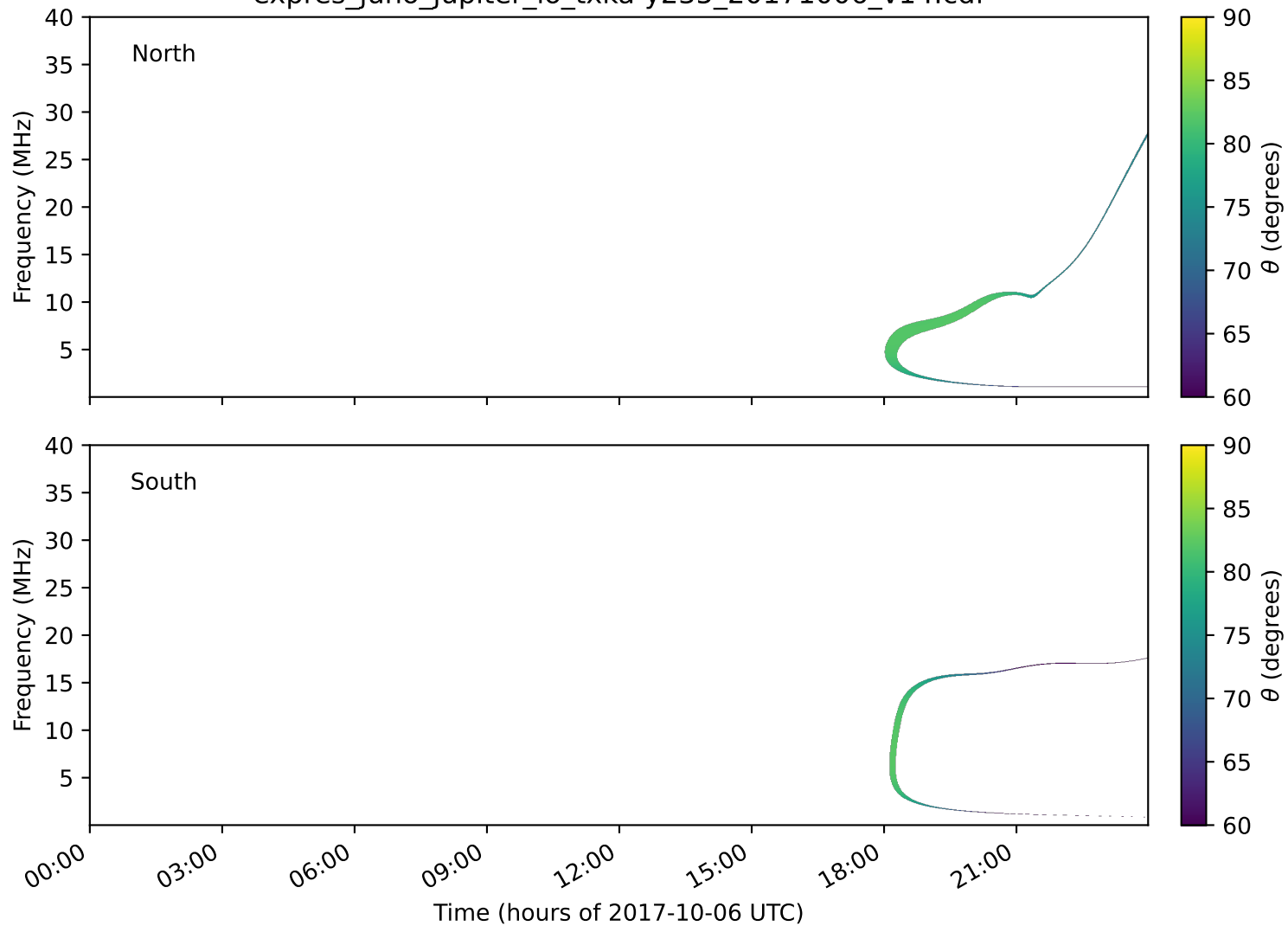
expres_juno_jupiter_io_txka-y235_20171006_v14.cdf
