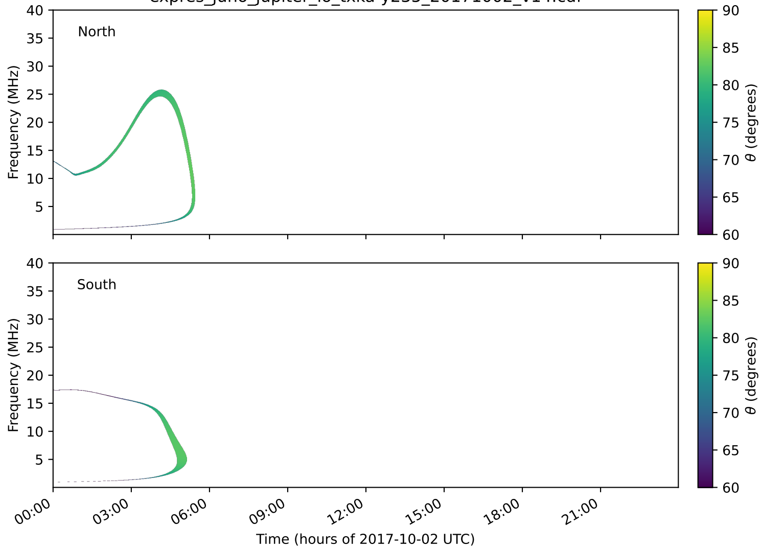
expres_juno_jupiter_io_txka-y235_20171002_v14.cdf
