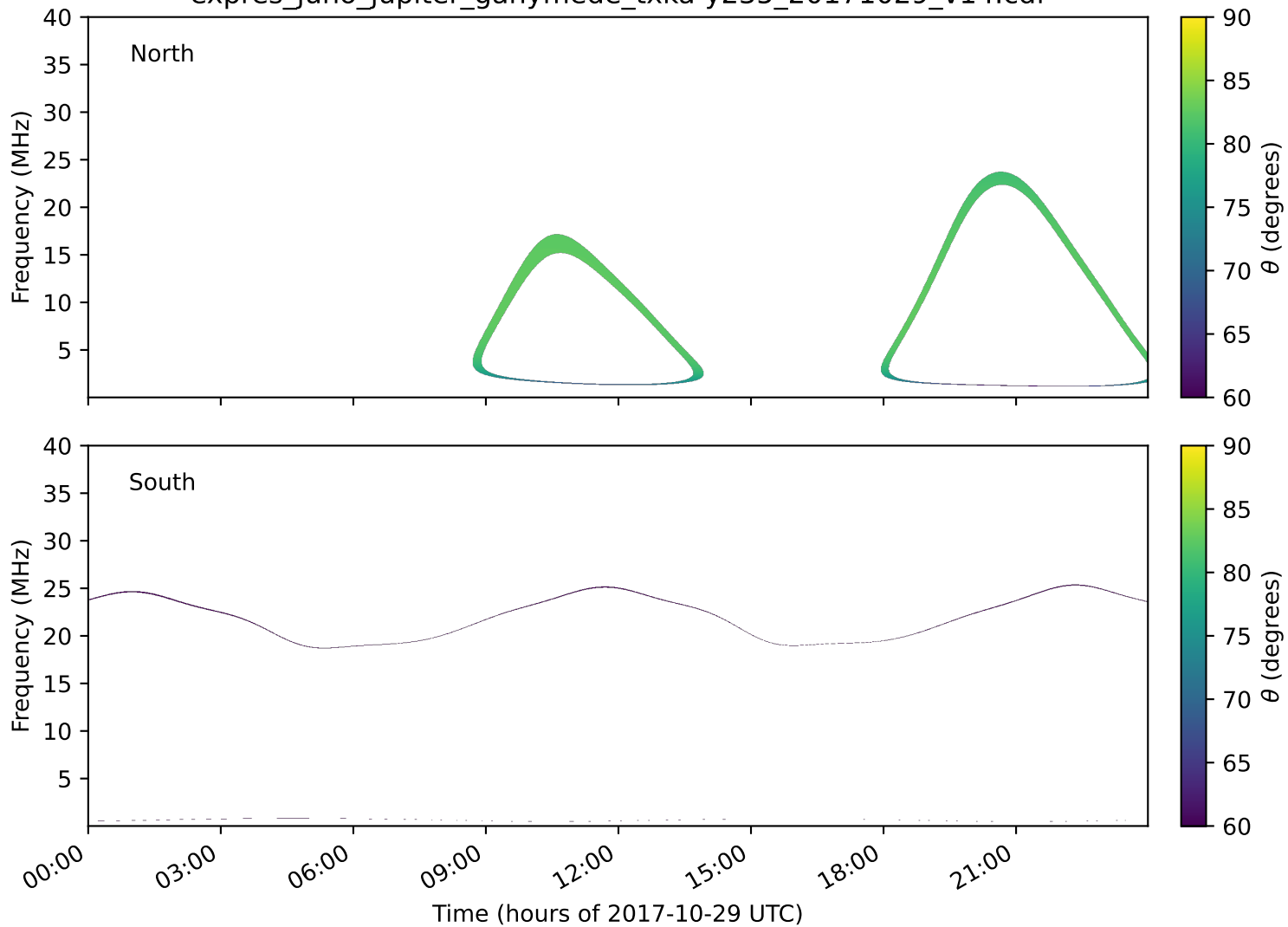
expres_juno_jupiter_ganymede_txka-y235_20171029_v14.cdf
