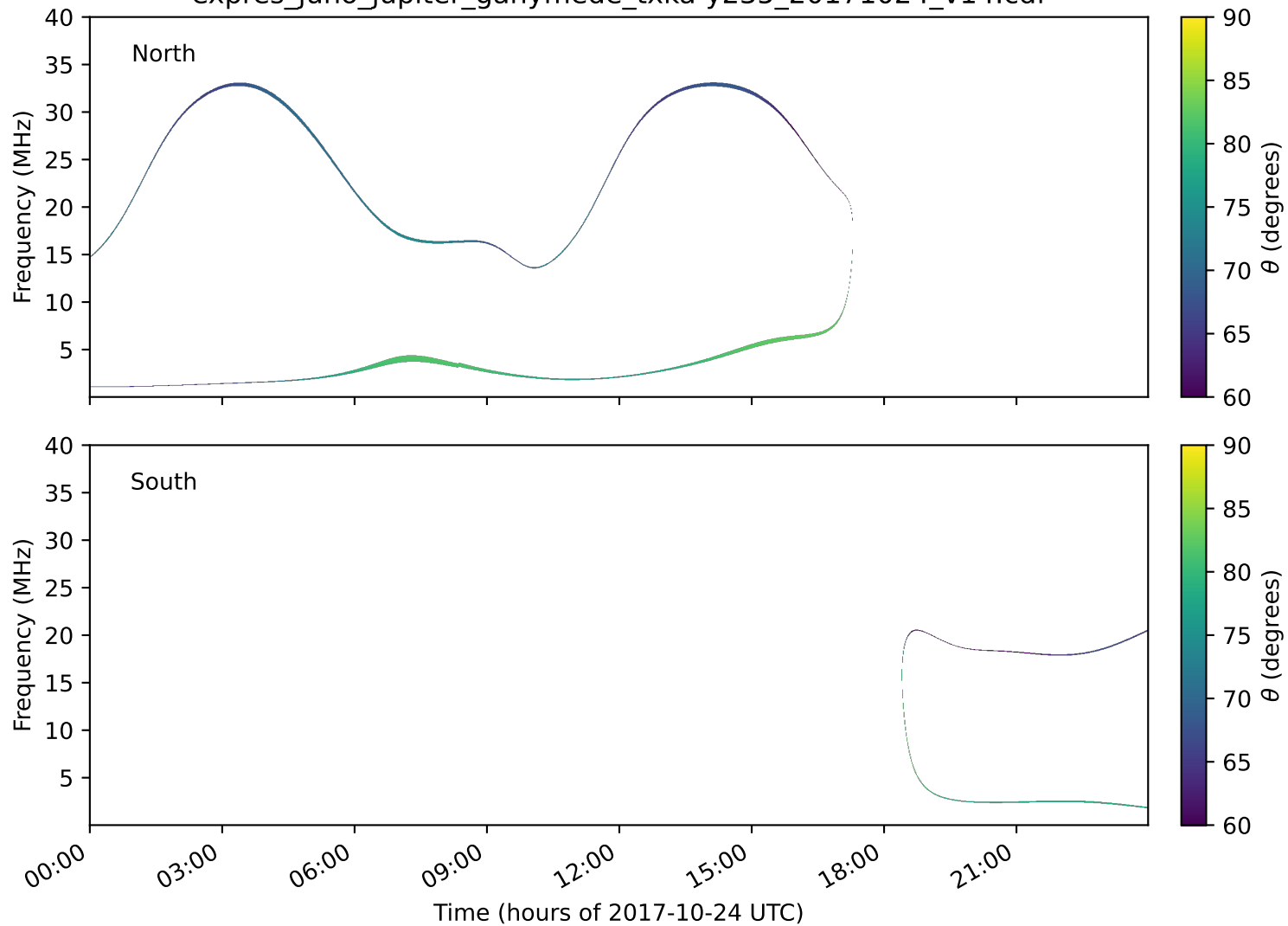
expres_juno_jupiter_ganymede_txka-y235_20171024_v14.cdf
