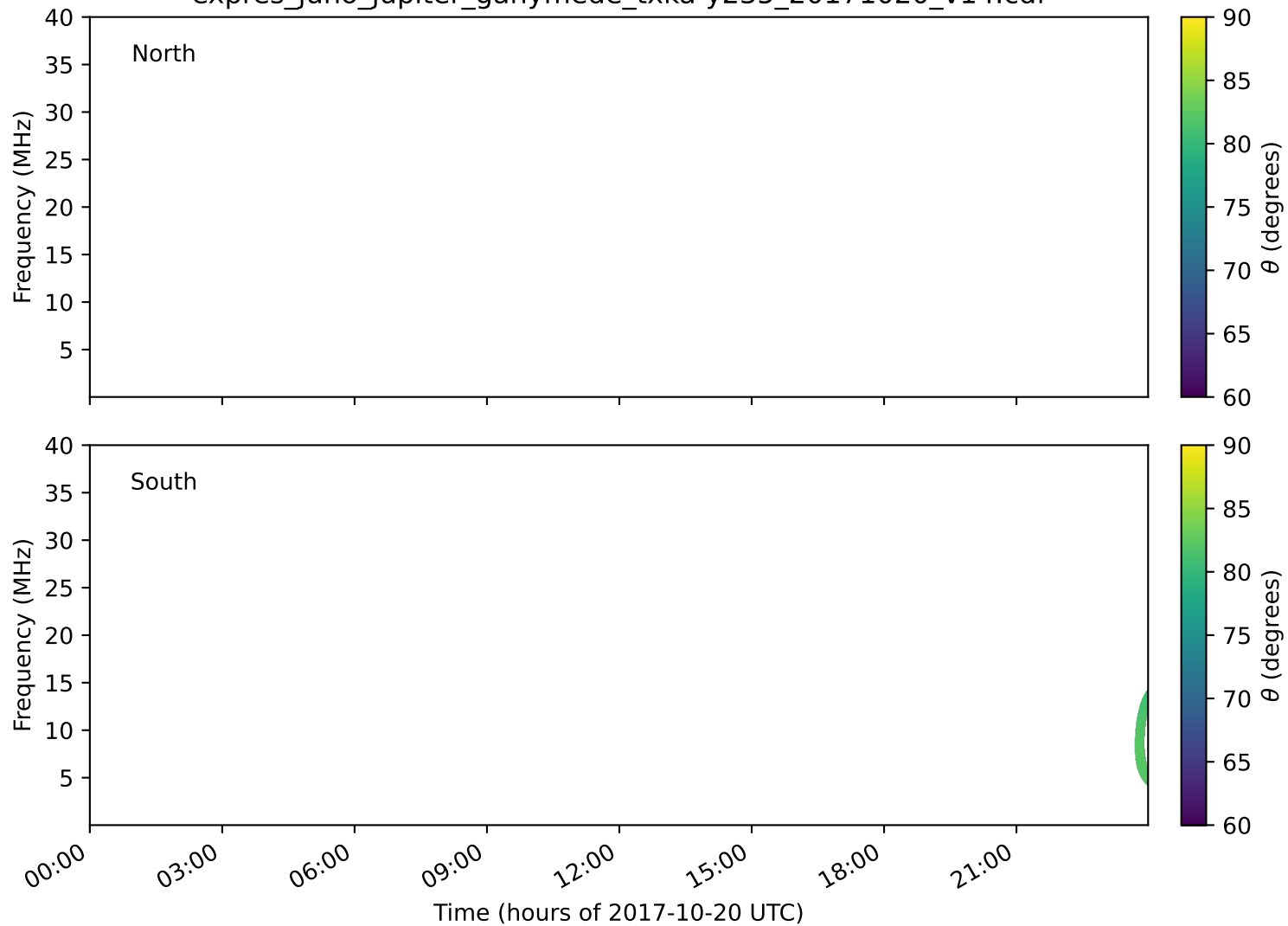
expres_juno_jupiter_ganymede_txka-y235_20171020_v14.cdf
