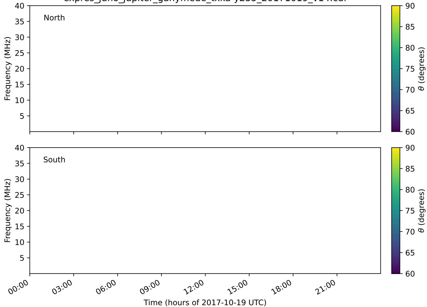
expres_juno_jupiter_ganymede_txka-y235_20171019_v14.cdf
