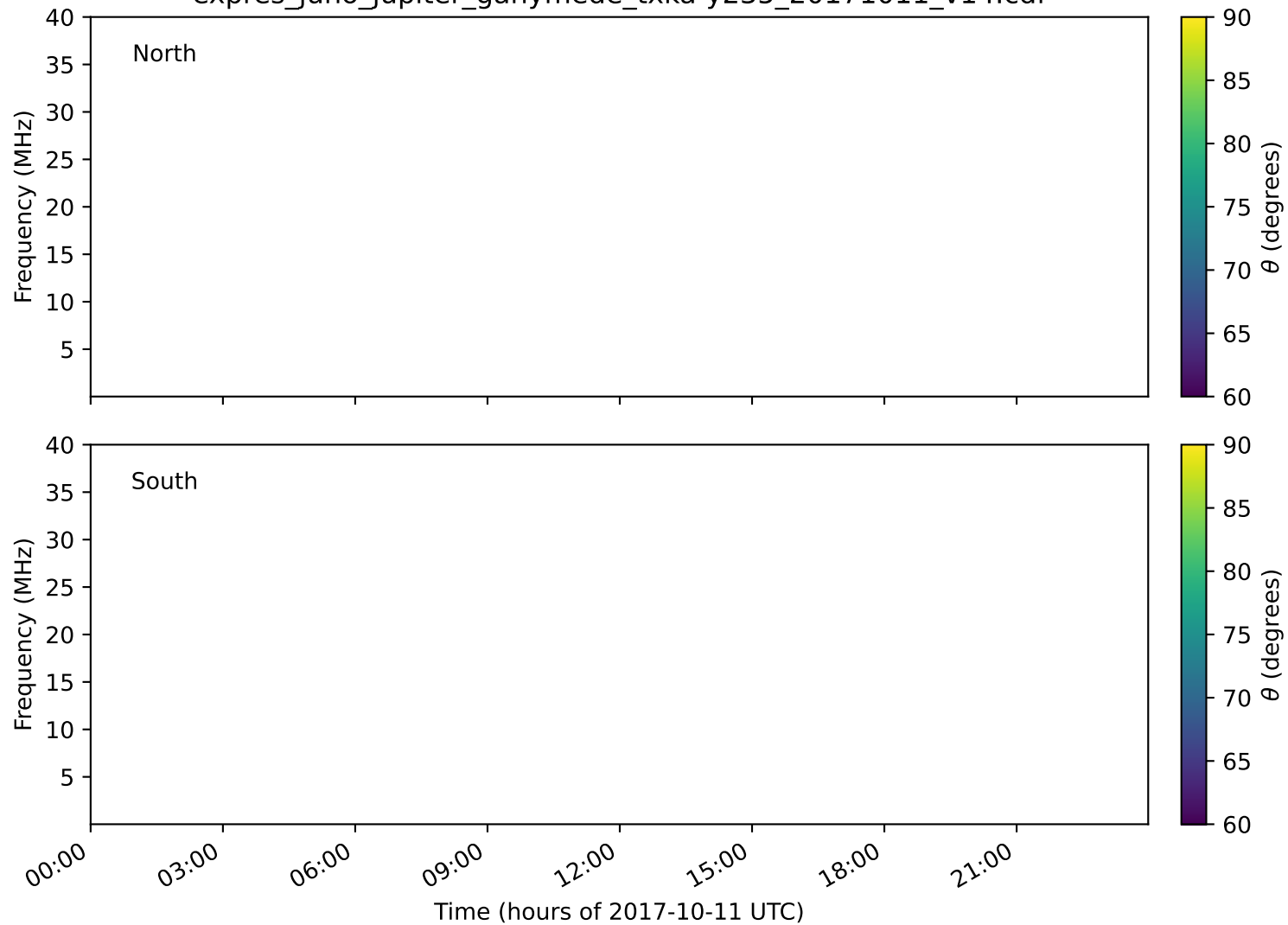
expres_juno_jupiter_ganymede_txka-y235_20171011_v14.cdf
