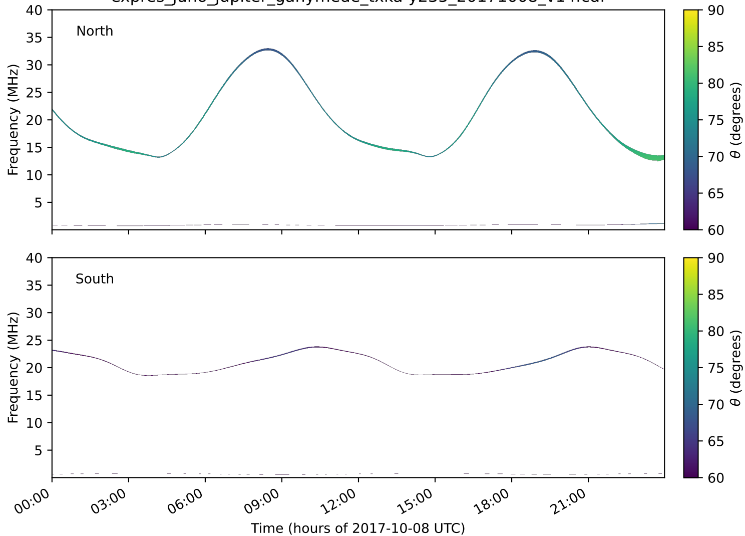
expres_juno_jupiter_ganymede_txka-y235_20171008_v14.cdf
