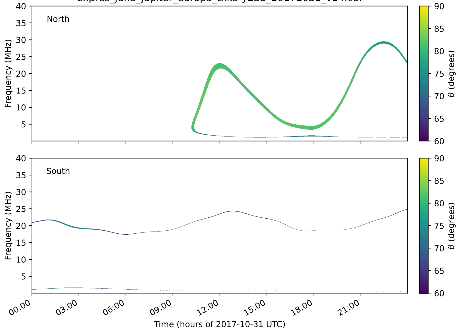
expres_juno_jupiter_europa_txka-y235_20171031_v14.cdf
