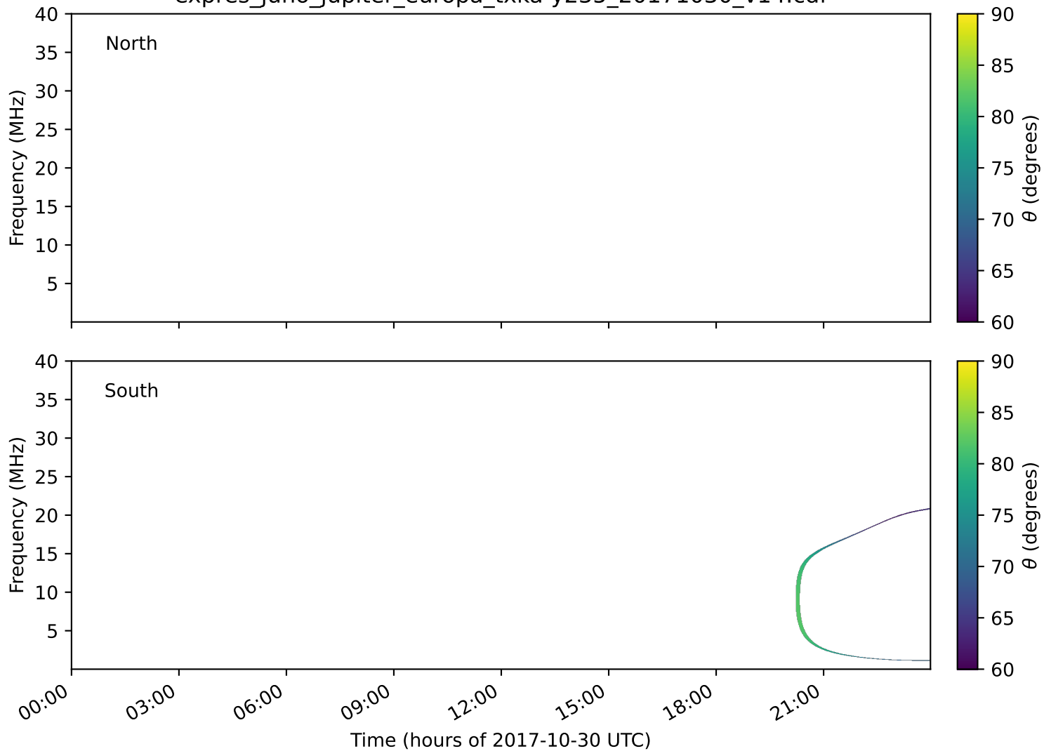
expres_juno_jupiter_europa_txka-y235_20171030_v14.cdf
