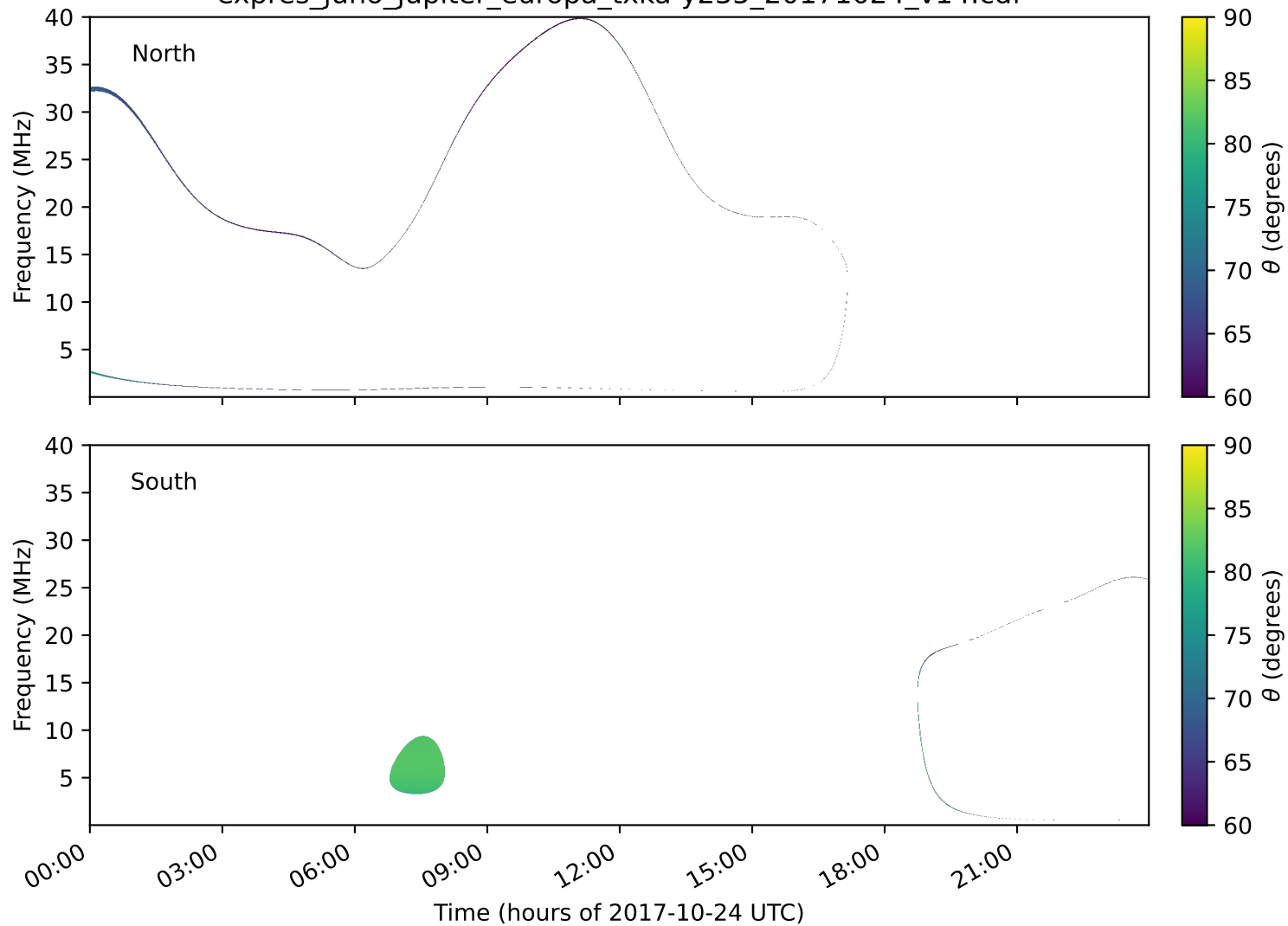
expres_juno_jupiter_europa_txka-y235_20171024_v14.cdf
