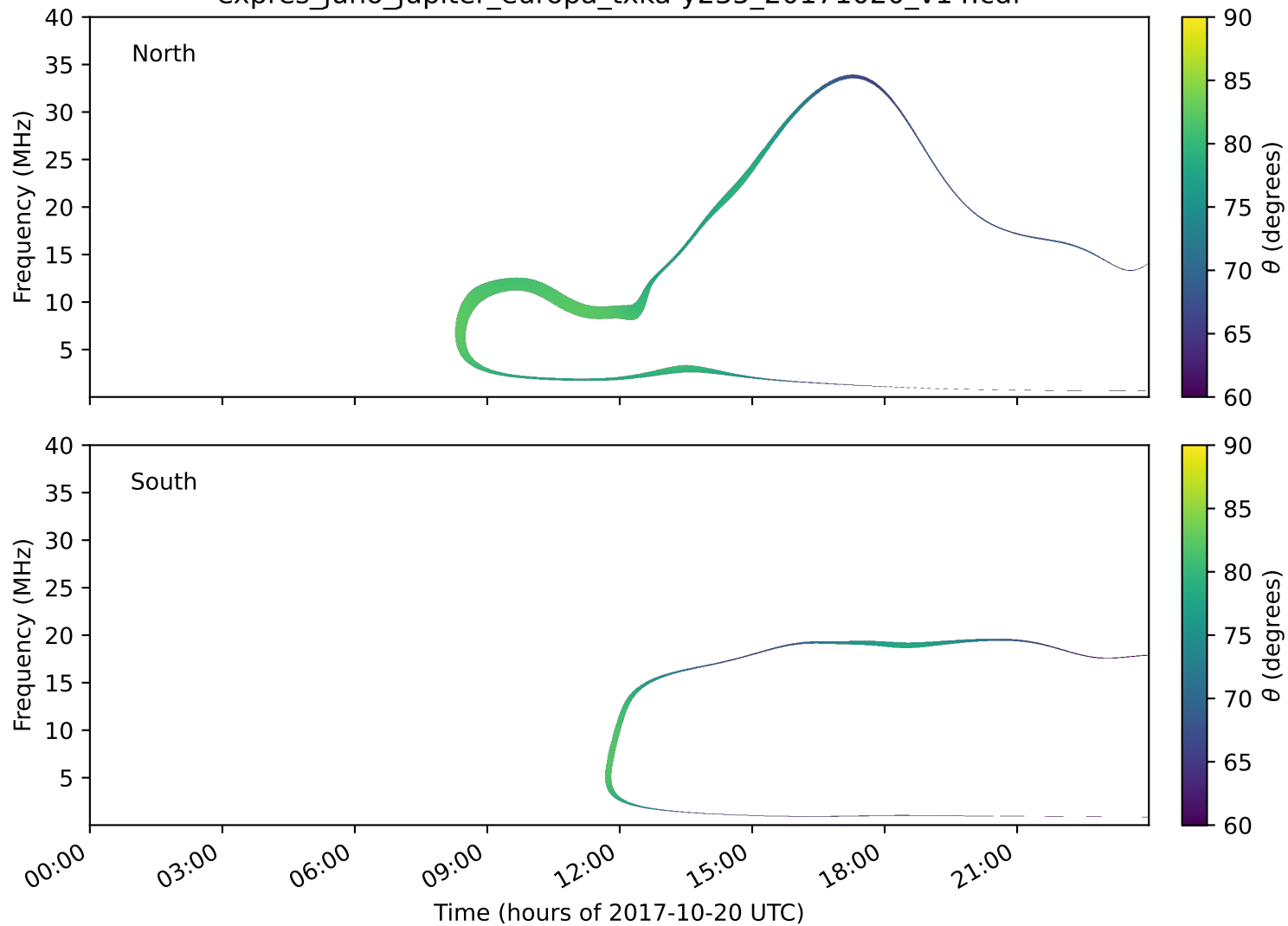
expres_juno_jupiter_europa_txka-y235_20171020_v14.cdf
