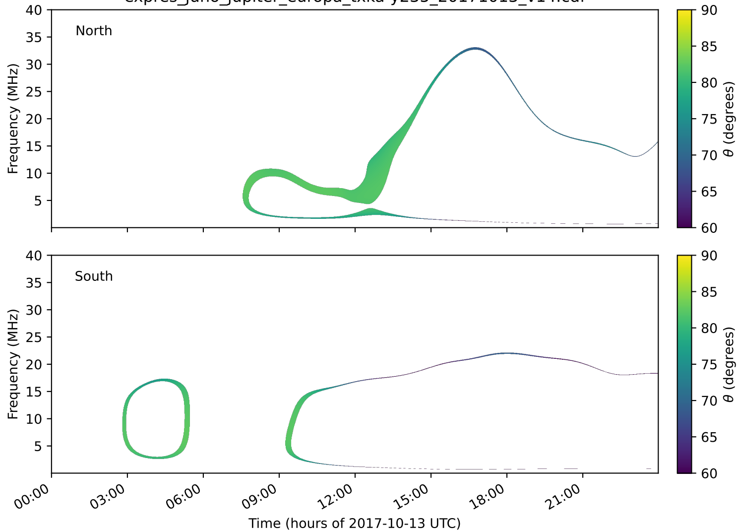
expres_juno_jupiter_europa_txka-y235_20171013_v14.cdf
