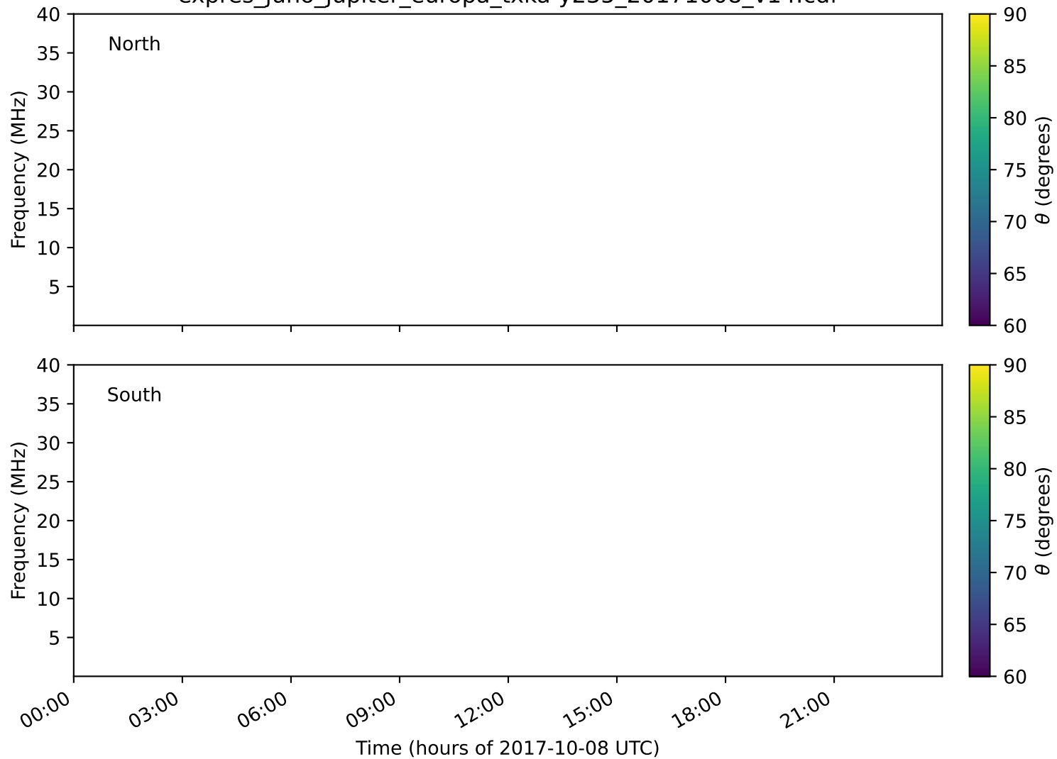
expres_juno_jupiter_europa_txka-y235_20171008_v14.cdf
