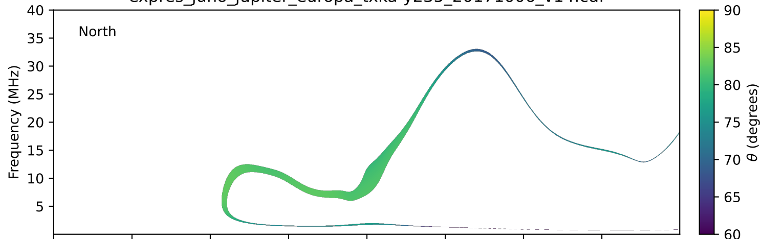
expres_juno_jupiter_europa_txka-y235_20171006_v14.cdf
