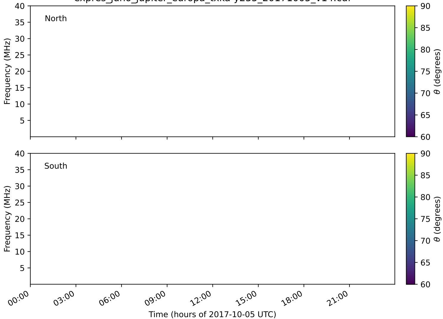
expres_juno_jupiter_europa_txka-y235_20171005_v14.cdf
