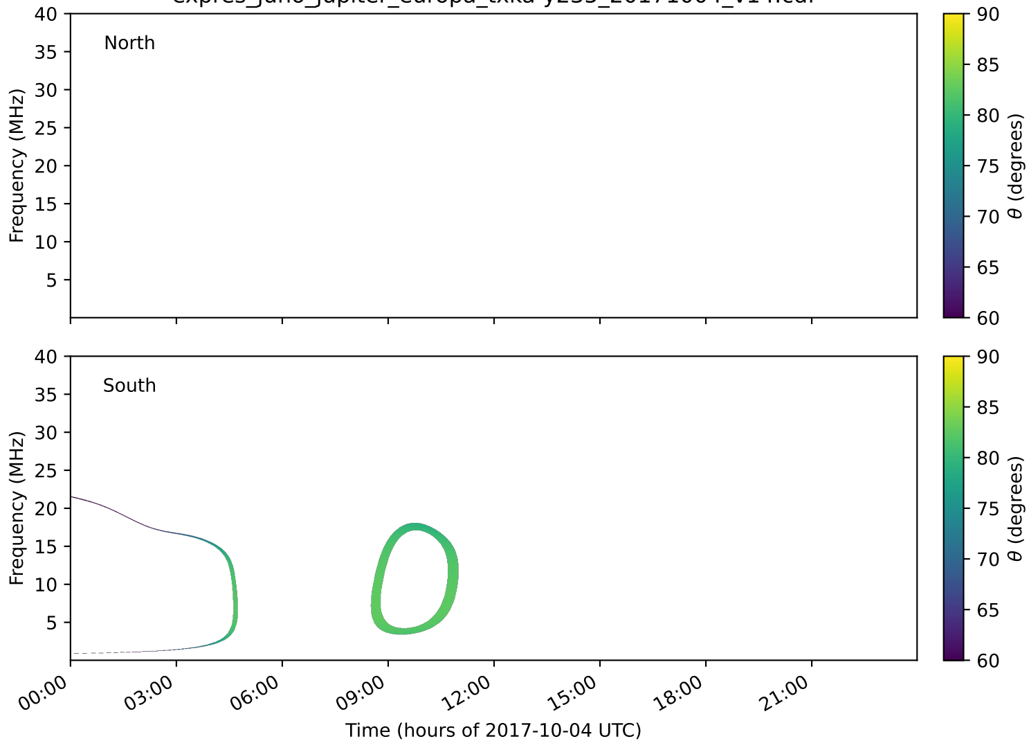
expres_juno_jupiter_europa_txka-y235_20171004_v14.cdf
