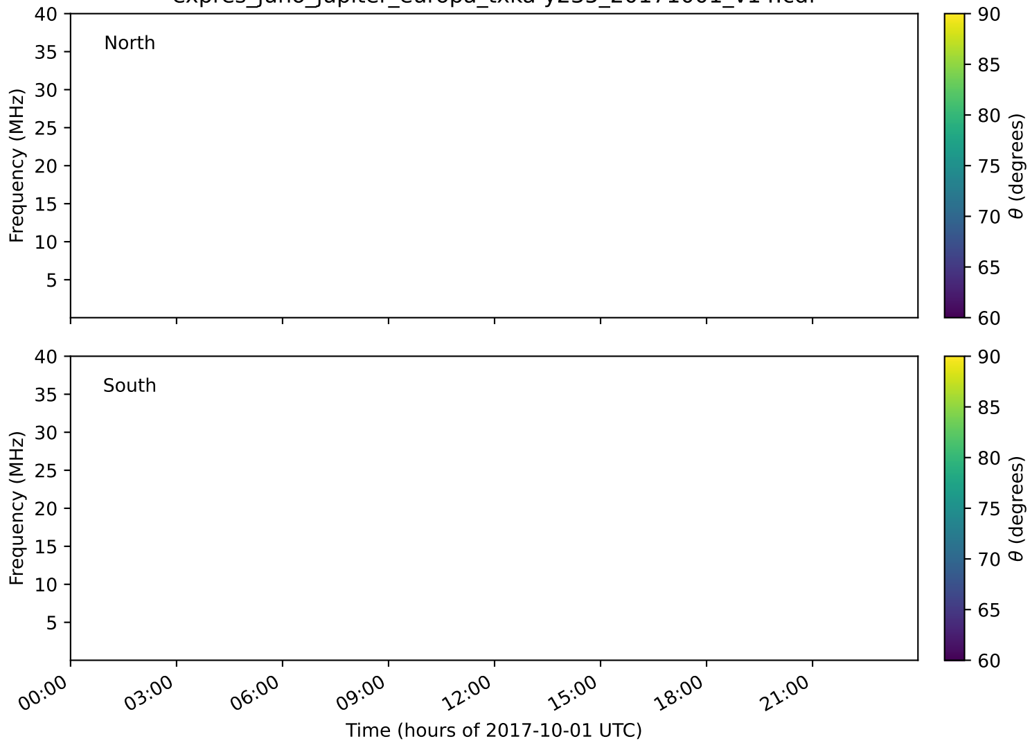
expres_juno_jupiter_europa_txka-y235_20171001_v14.cdf
