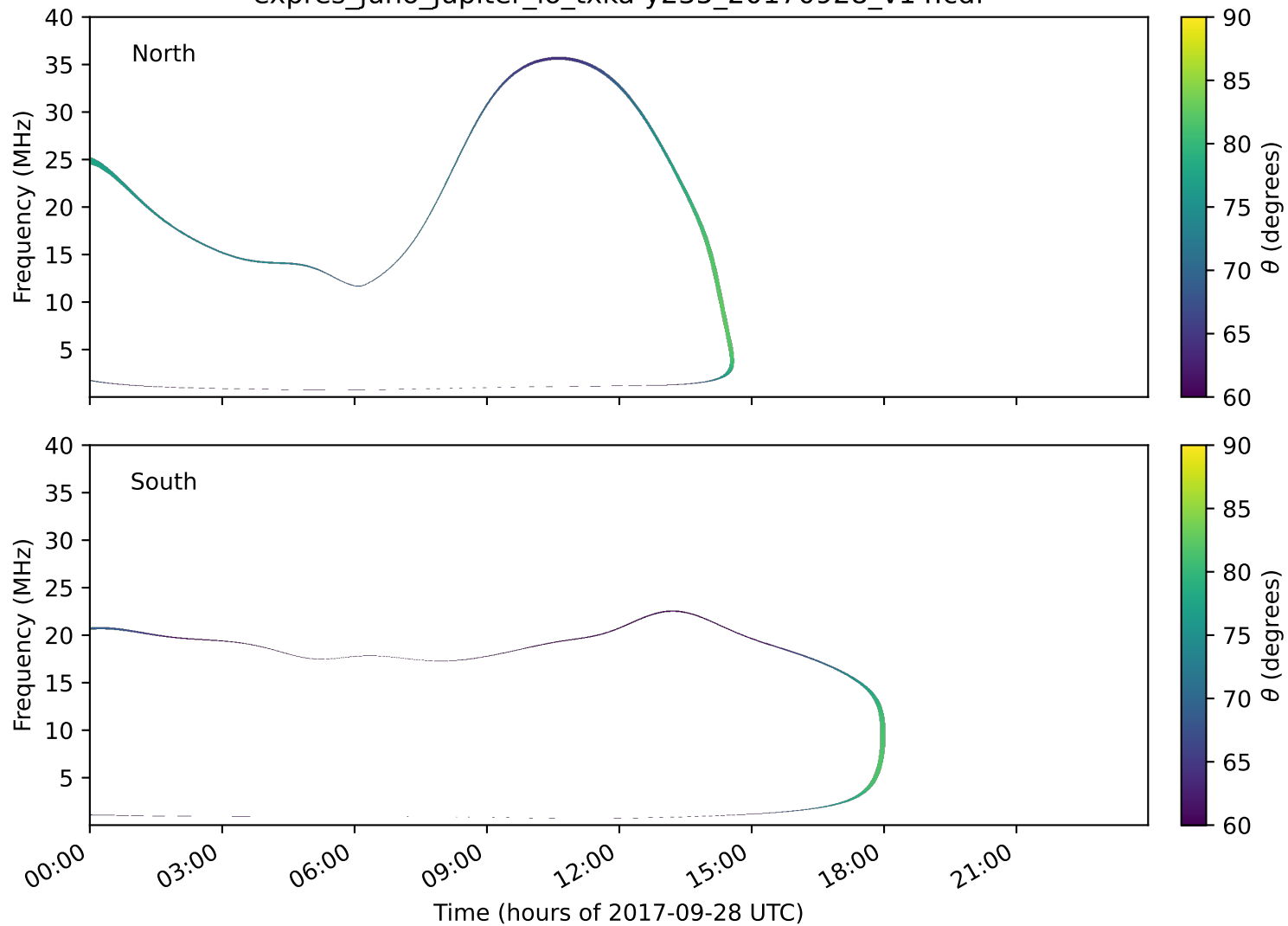
expres_juno_jupiter_io_txka-y235_20170928_v14.cdf
