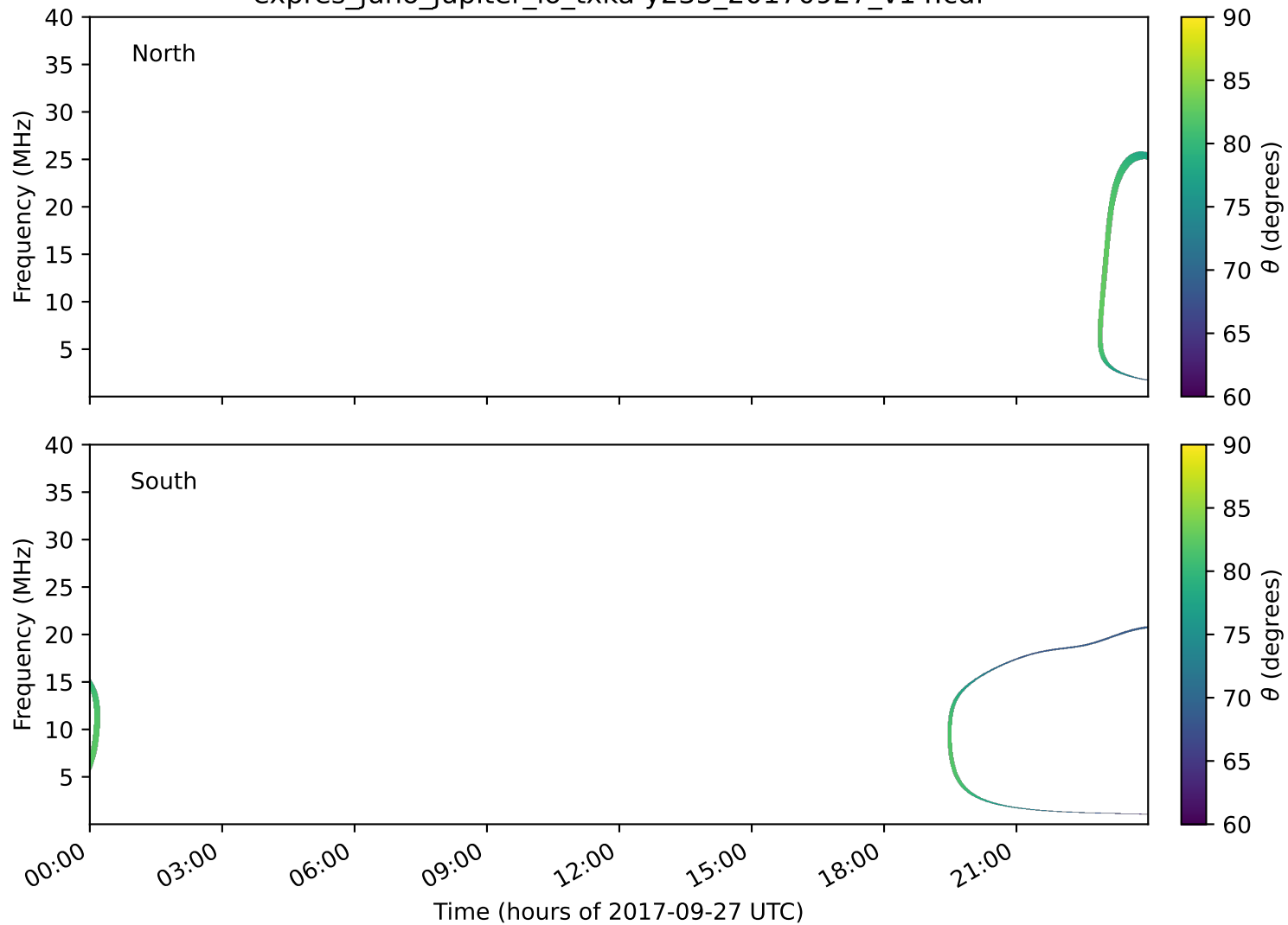
expres_juno_jupiter_io_txka-y235_20170927_v14.cdf
