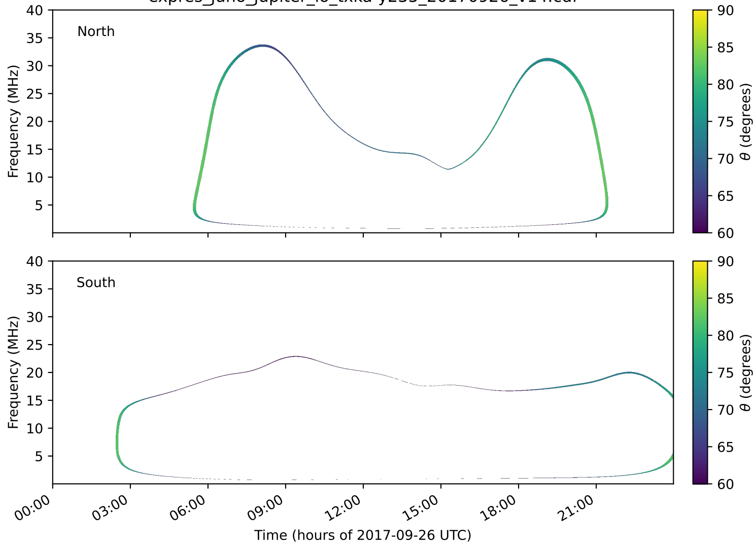
expres_juno_jupiter_io_txka-y235_20170926_v14.cdf
