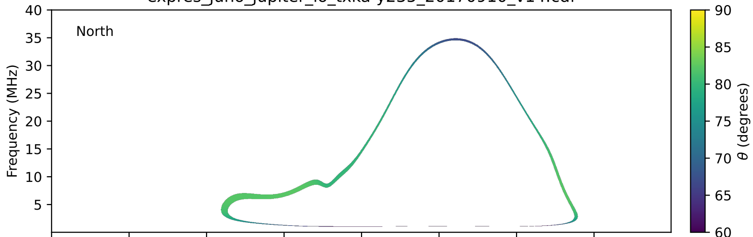
expres_juno_jupiter_io_txka-y235_20170910_v14.cdf
