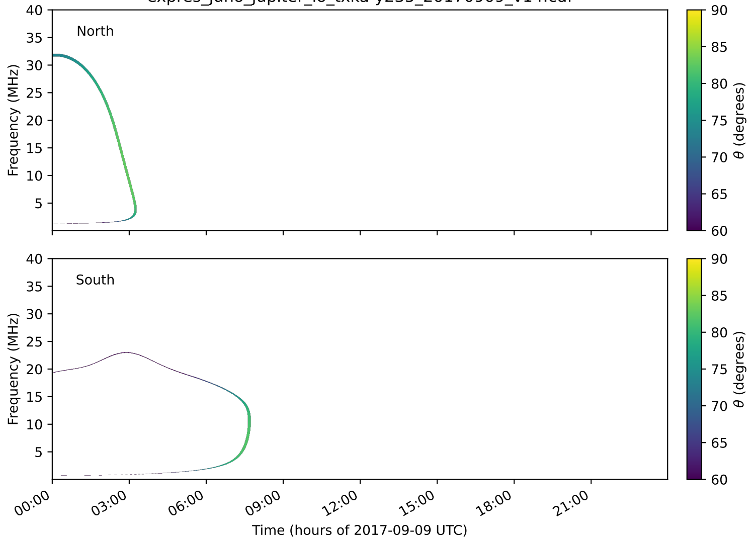
expres_juno_jupiter_io_txka-y235_20170909_v14.cdf
