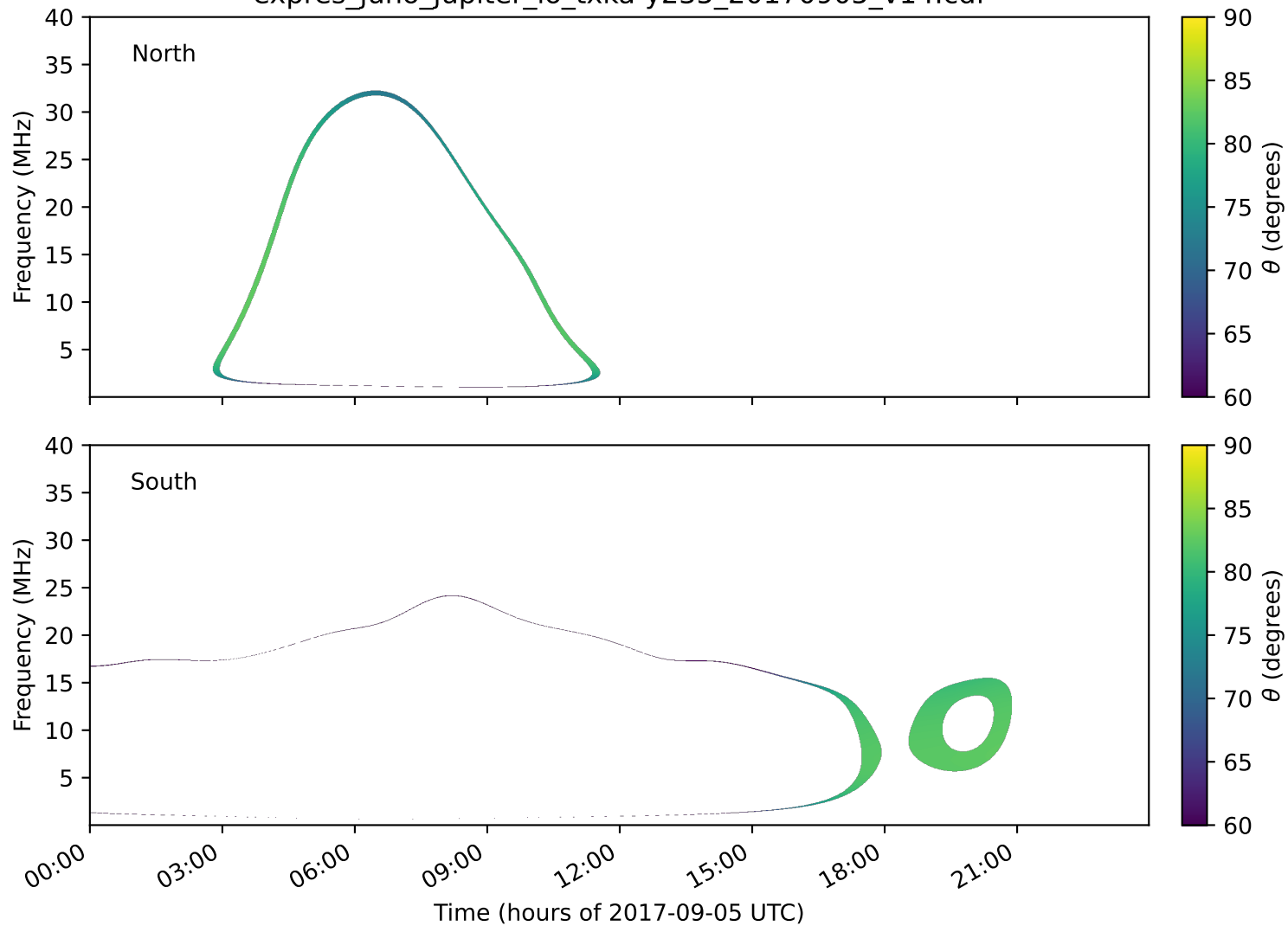
expres_juno_jupiter_io_txka-y235_20170905_v14.cdf
