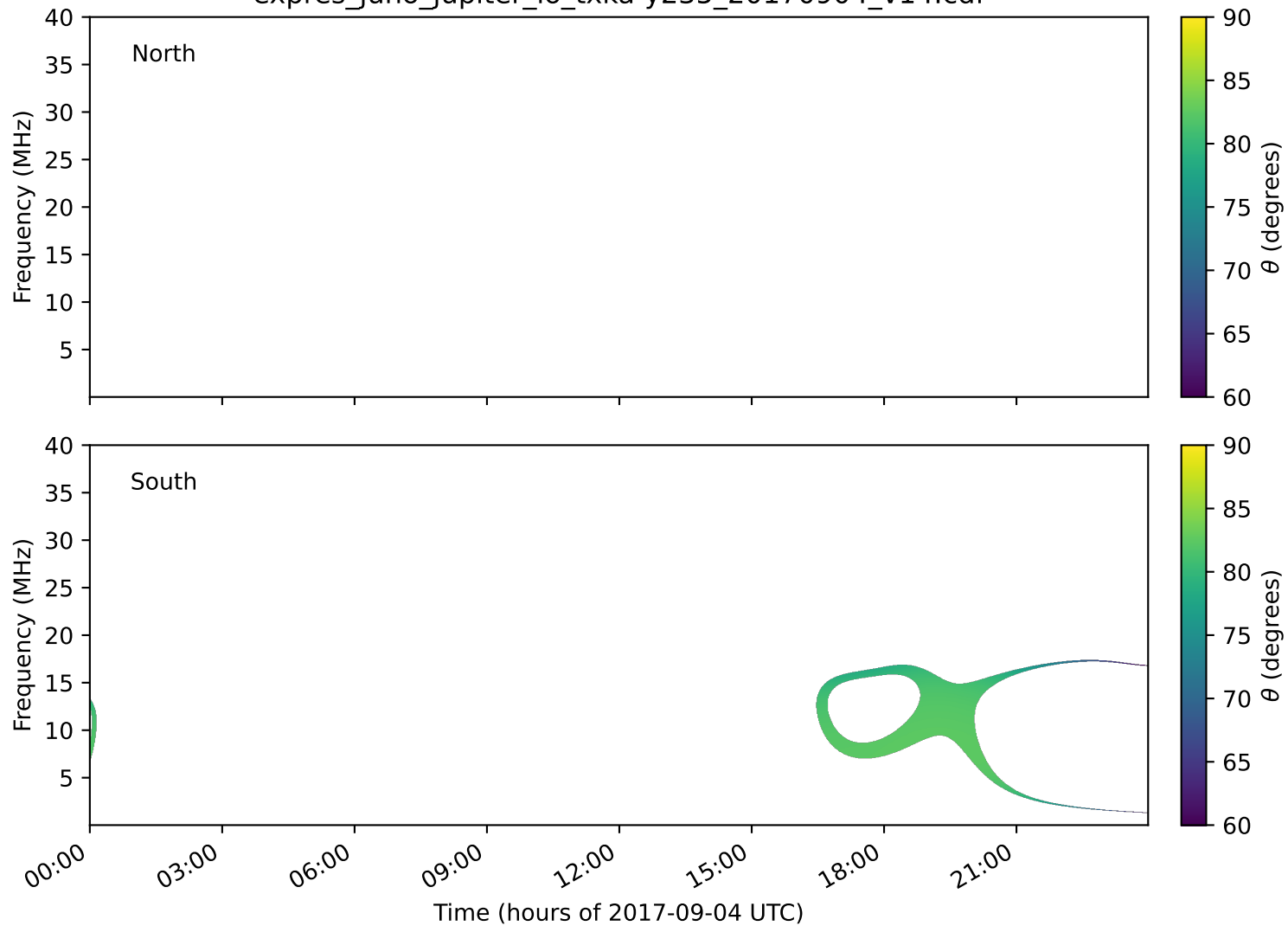
expres_juno_jupiter_io_txka-y235_20170904_v14.cdf
