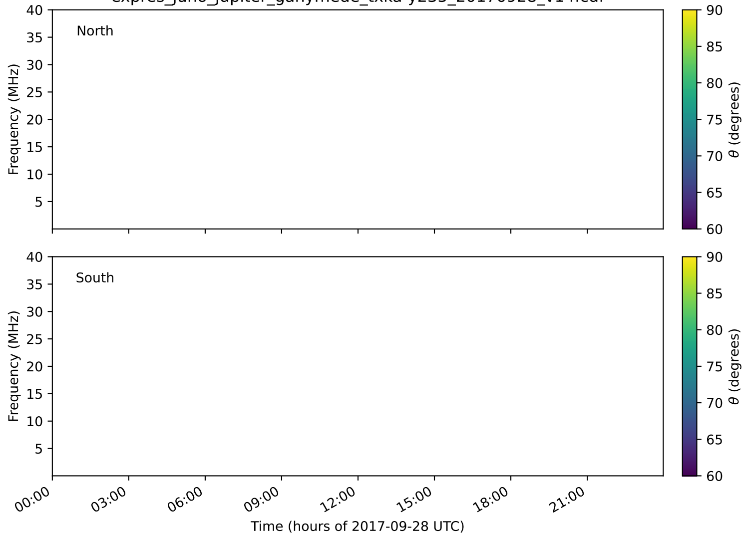
expres_juno_jupiter_ganymede_txka-y235_20170928_v14.cdf
