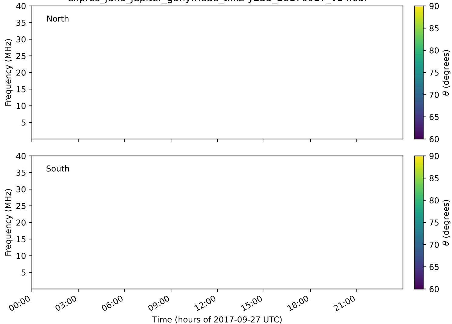
expres_juno_jupiter_ganymede_txka-y235_20170927_v14.cdf
