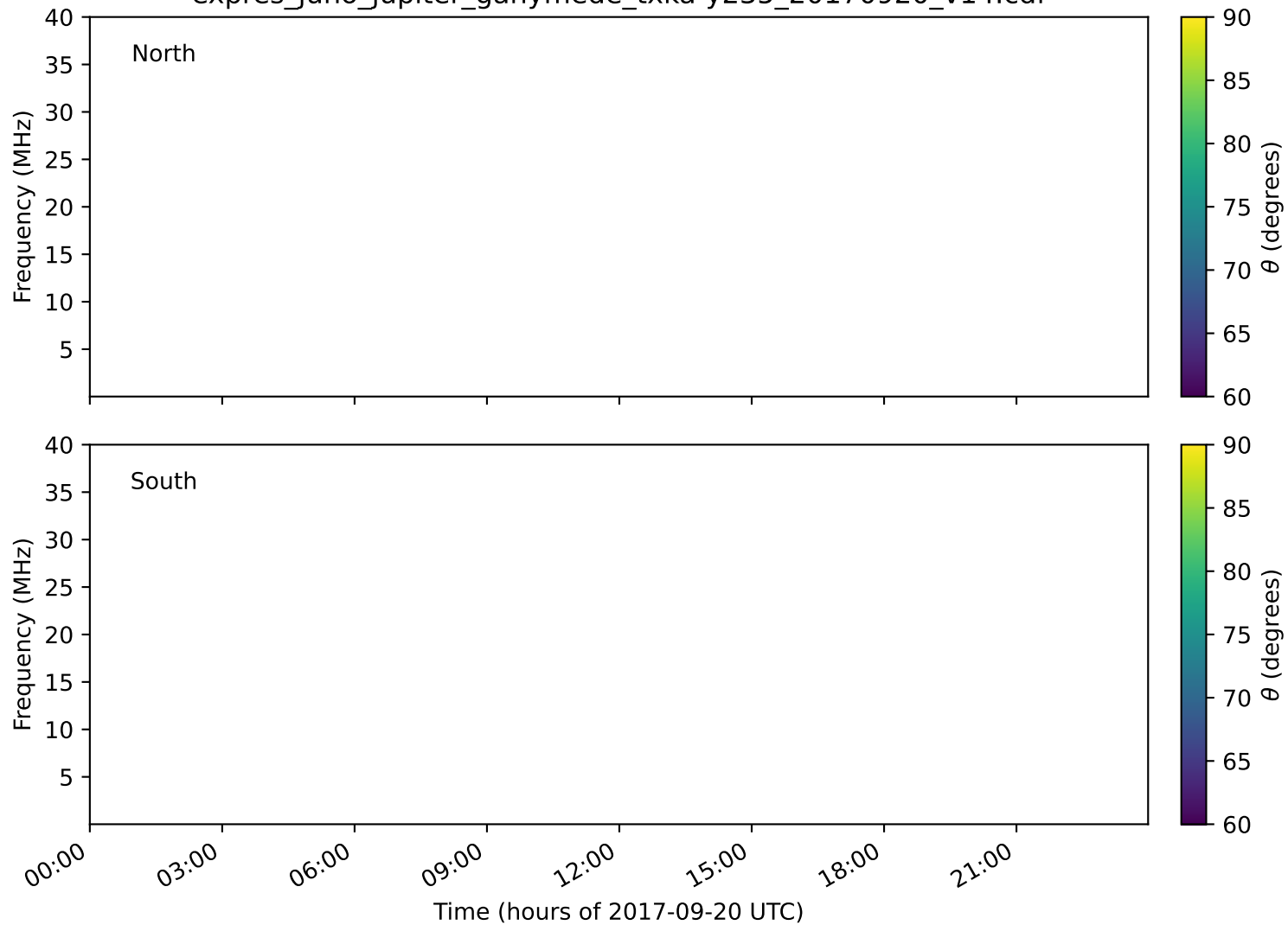
expres_juno_jupiter_ganymede_txka-y235_20170920_v14.cdf
