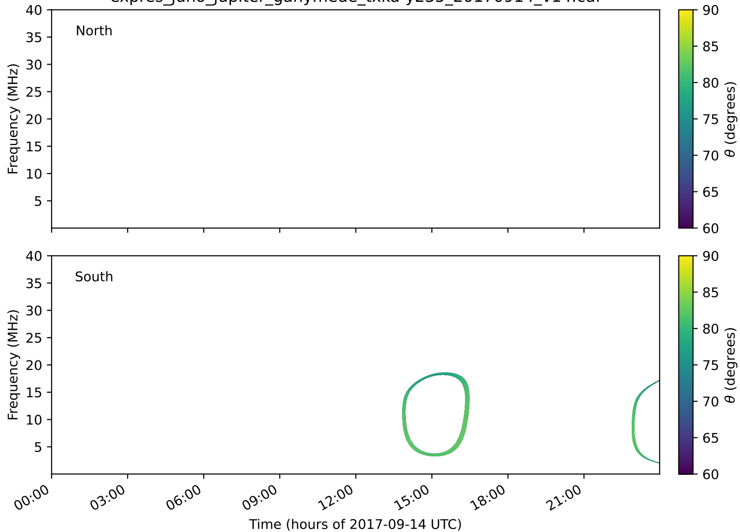
expres_juno_jupiter_ganymede_txka-y235_20170914_v14.cdf
