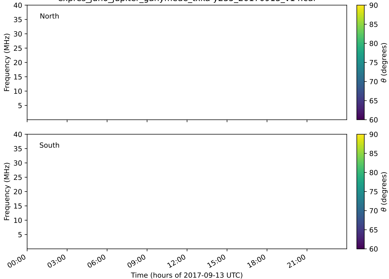
expres_juno_jupiter_ganymede_txka-y235_20170913_v14.cdf
