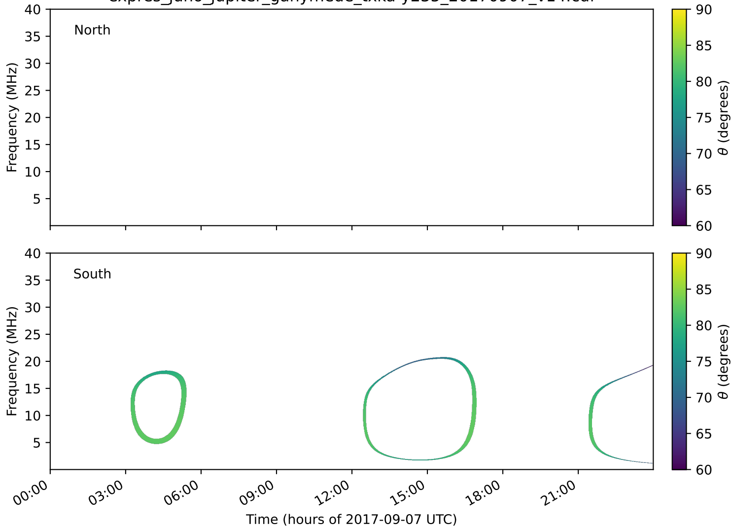
expres_juno_jupiter_ganymede_txka-y235_20170907_v14.cdf
