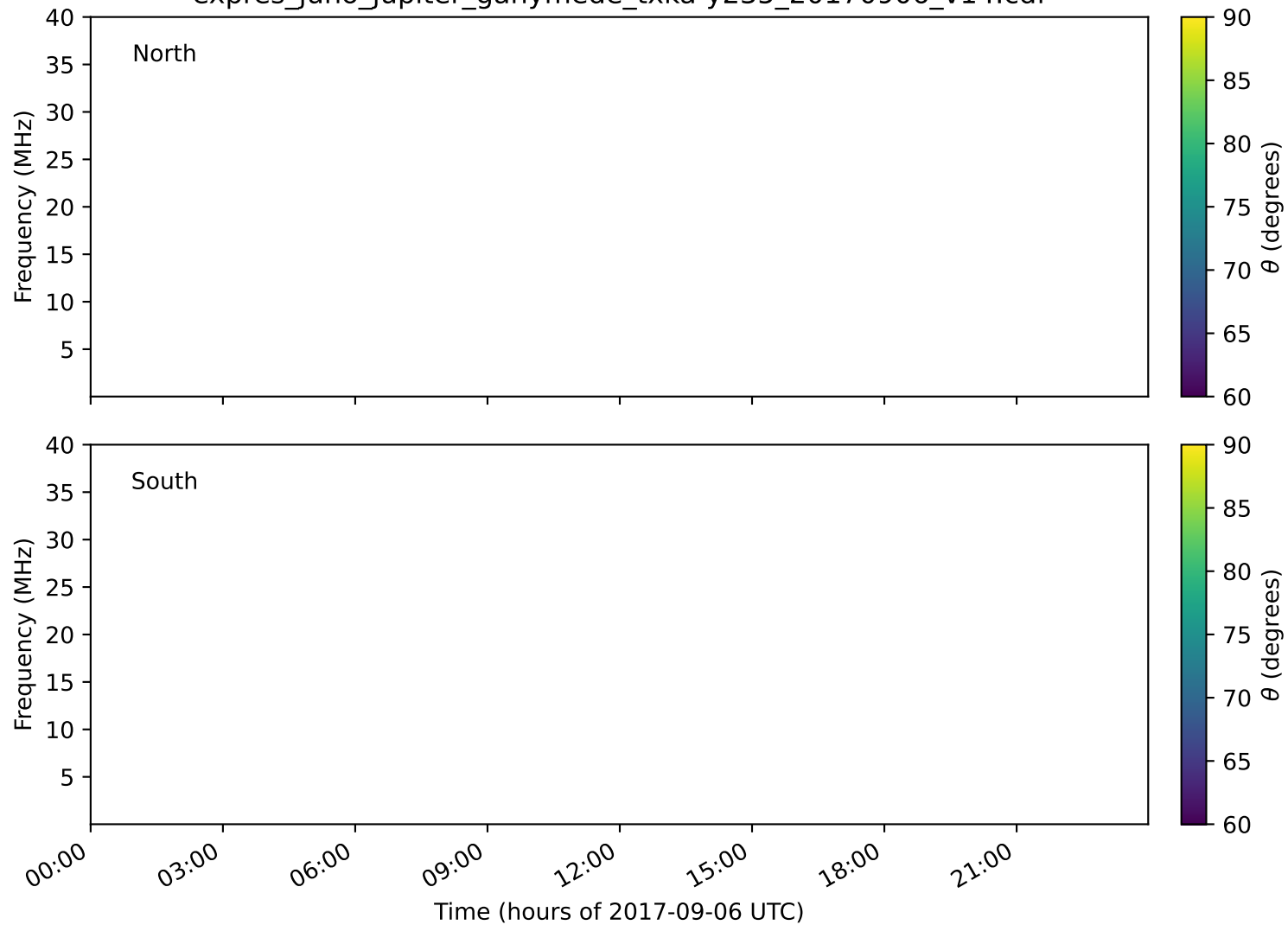
expres_juno_jupiter_ganymede_txka-y235_20170906_v14.cdf
