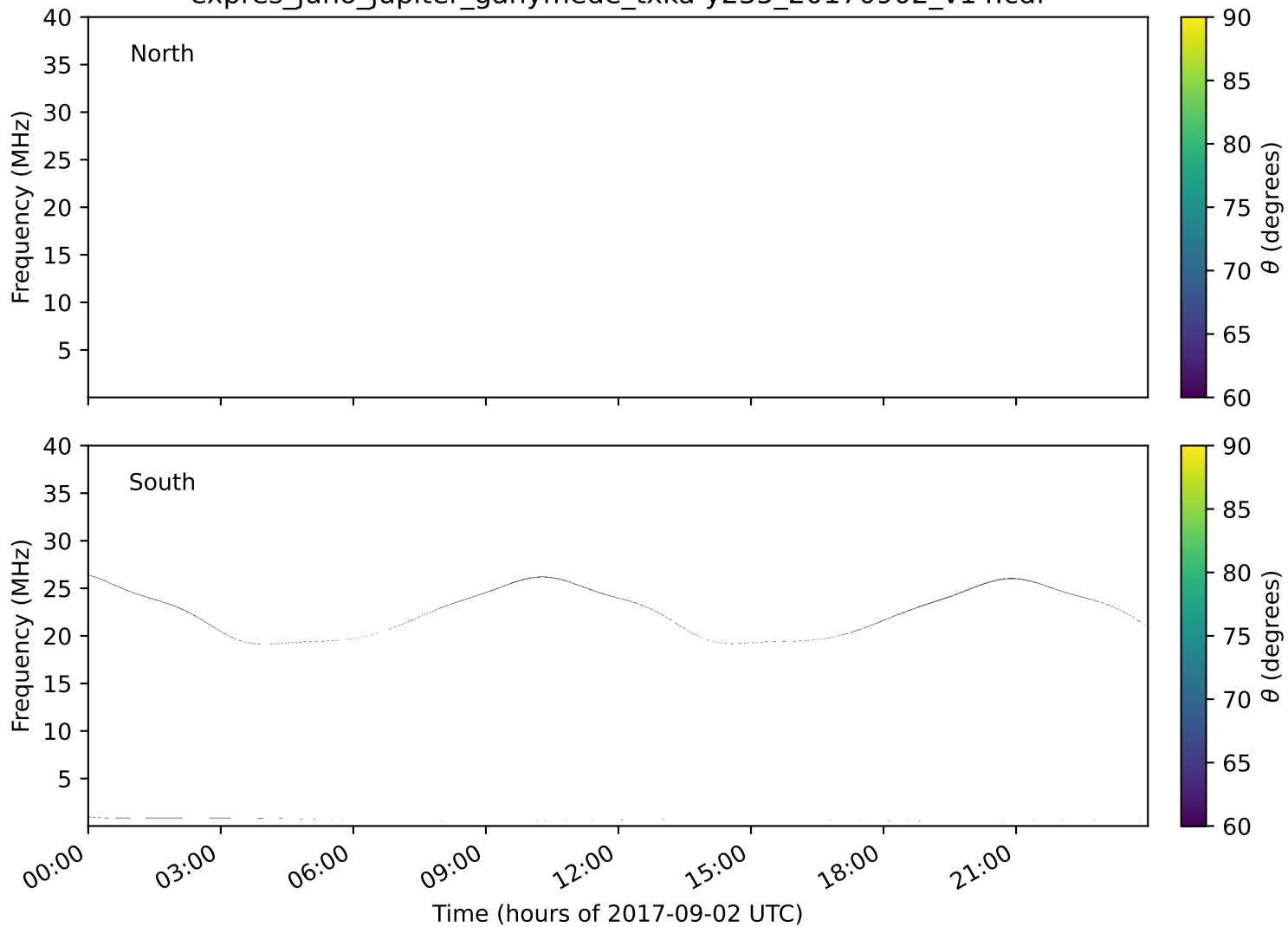
expres_juno_jupiter_ganymede_txka-y235_20170902_v14.cdf
