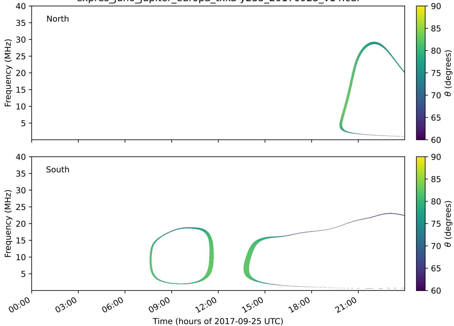
expres_juno_jupiter_europa_txka-y235_20170925_v14.cdf
