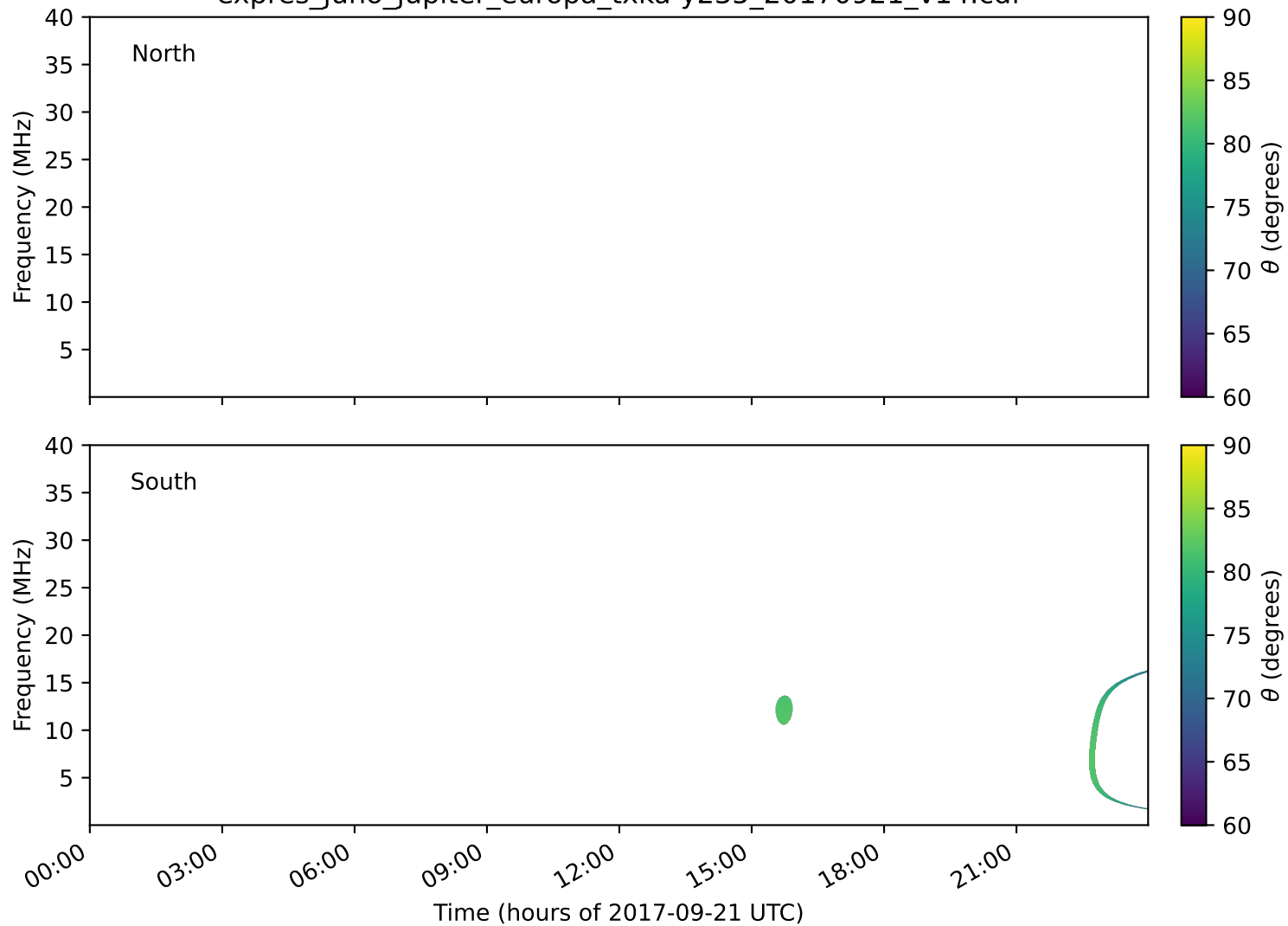
expres_juno_jupiter_europa_txka-y235_20170921_v14.cdf
